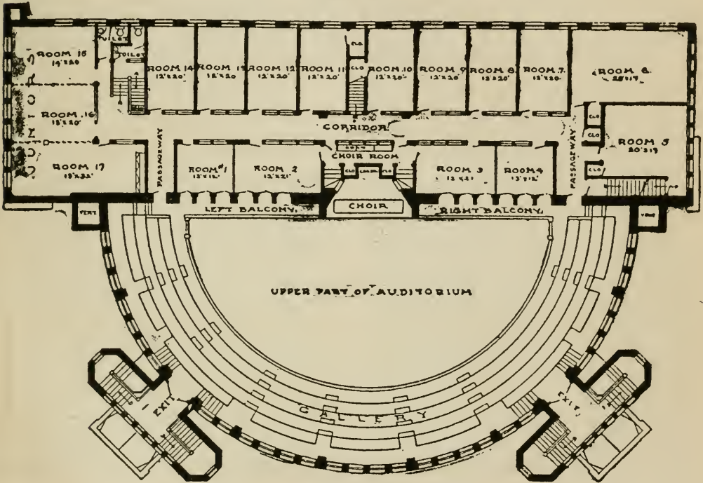
SECOND STORY PLAN ST. PAUL'S M. E. CHURCH, CEDAR RAPIDS, IA.
